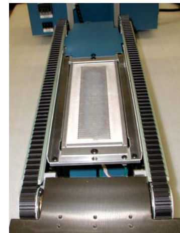
Lower Heater Assembly with Side Heat Shields
